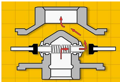
D. Single monitor operation, one full internal diaphragm case failure
