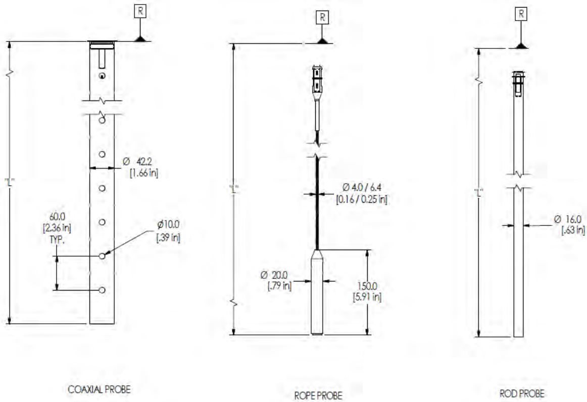
Figure 30 - SLG726 Probes
