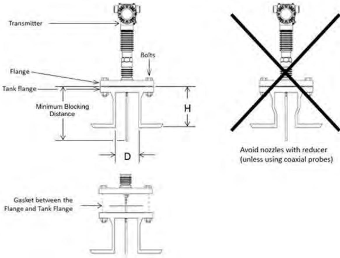
Figure 13 - Flange mounting
