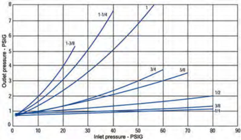
B-38R Relief Curves – Blocked Per Orifice 14" w.c. Set Point
