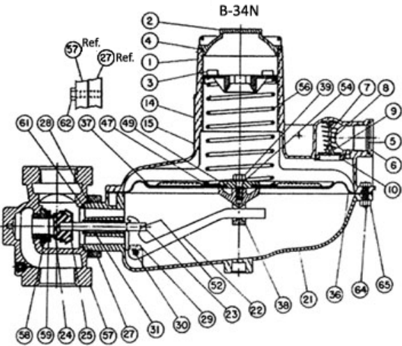
B34N Reference Schematic
