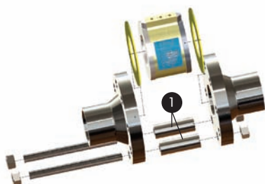
1 Centering Tubes
